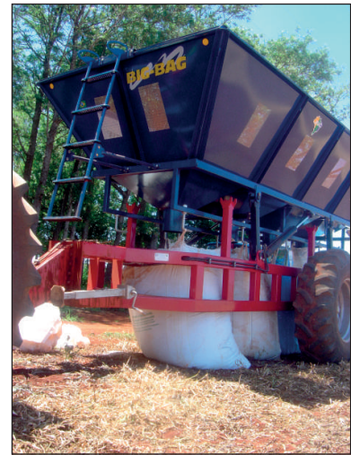
Big Bag 4 Spouts | Big Bag 4 Boquillas
